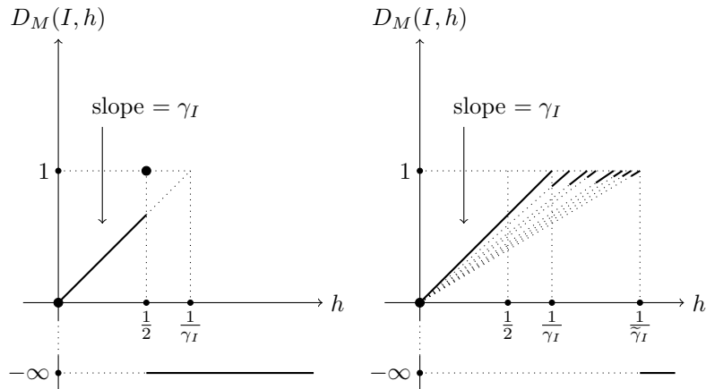
FIGURE 2. Local multifractal spectrum of M in the interval I when \sigma \neq 0 (left) and \sigma \equiv 0 (right). The right figure is a representation, since there is a countable number of small affine parts. When \sigma \neq 0 , the Brownian integral "hides" the complicated right part of D_M(I, \cdot) .
