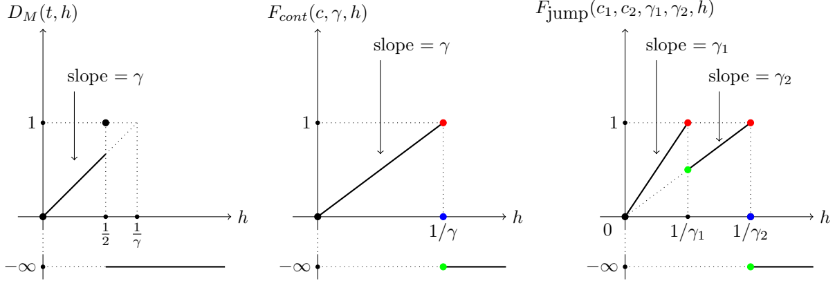
FIGURE 1. Pointwise multifractal spectra of M . Left: \sigma \neq 0 . Center: \sigma = 0 and t is a continuous time. Right: \sigma = 0 and t is a jump time. See the statement of Theorem 1 and 2 for the value of \gamma , \gamma_1 and \gamma_2 . The colored points correspond to possible values for the discontinuities of the pointwise spectra.
